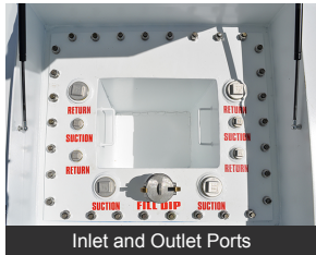
Inlet and Outlet Ports
